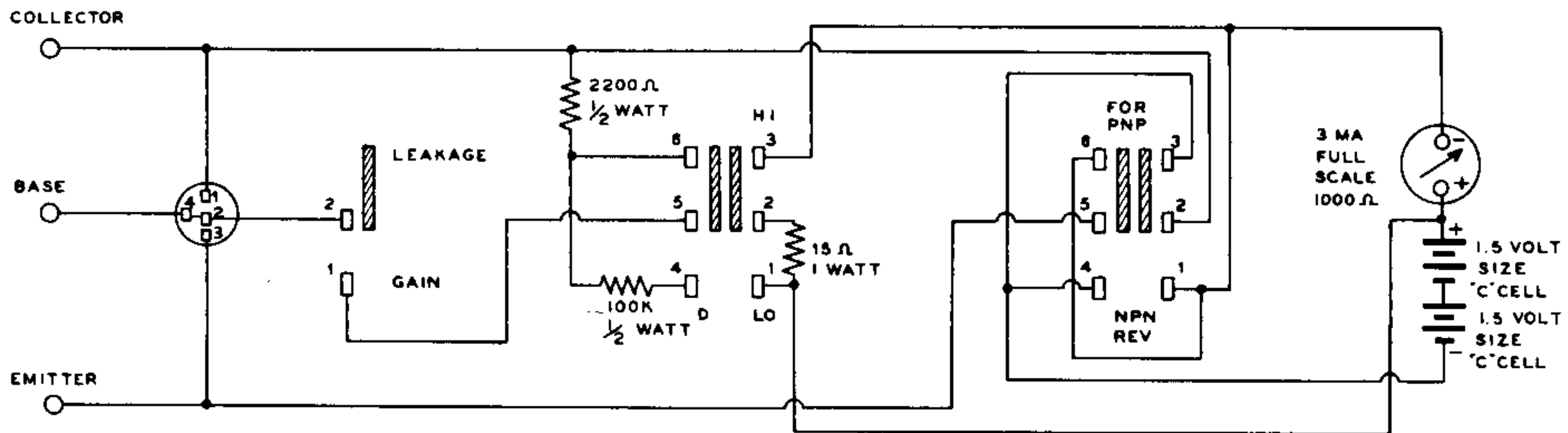
SCHMATIC DIAGRAM
