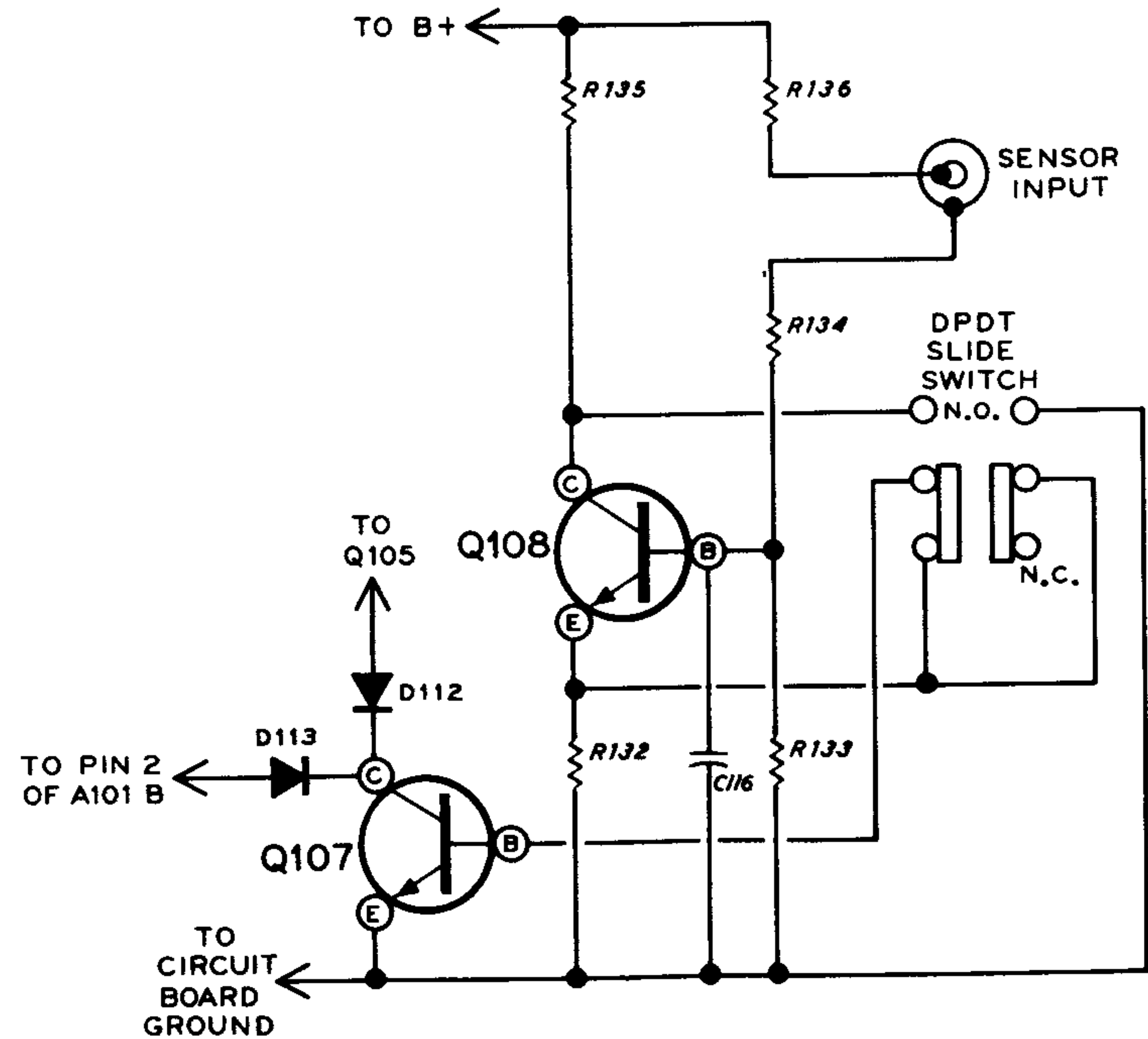
Figure 6 (Normally closed contacts)
