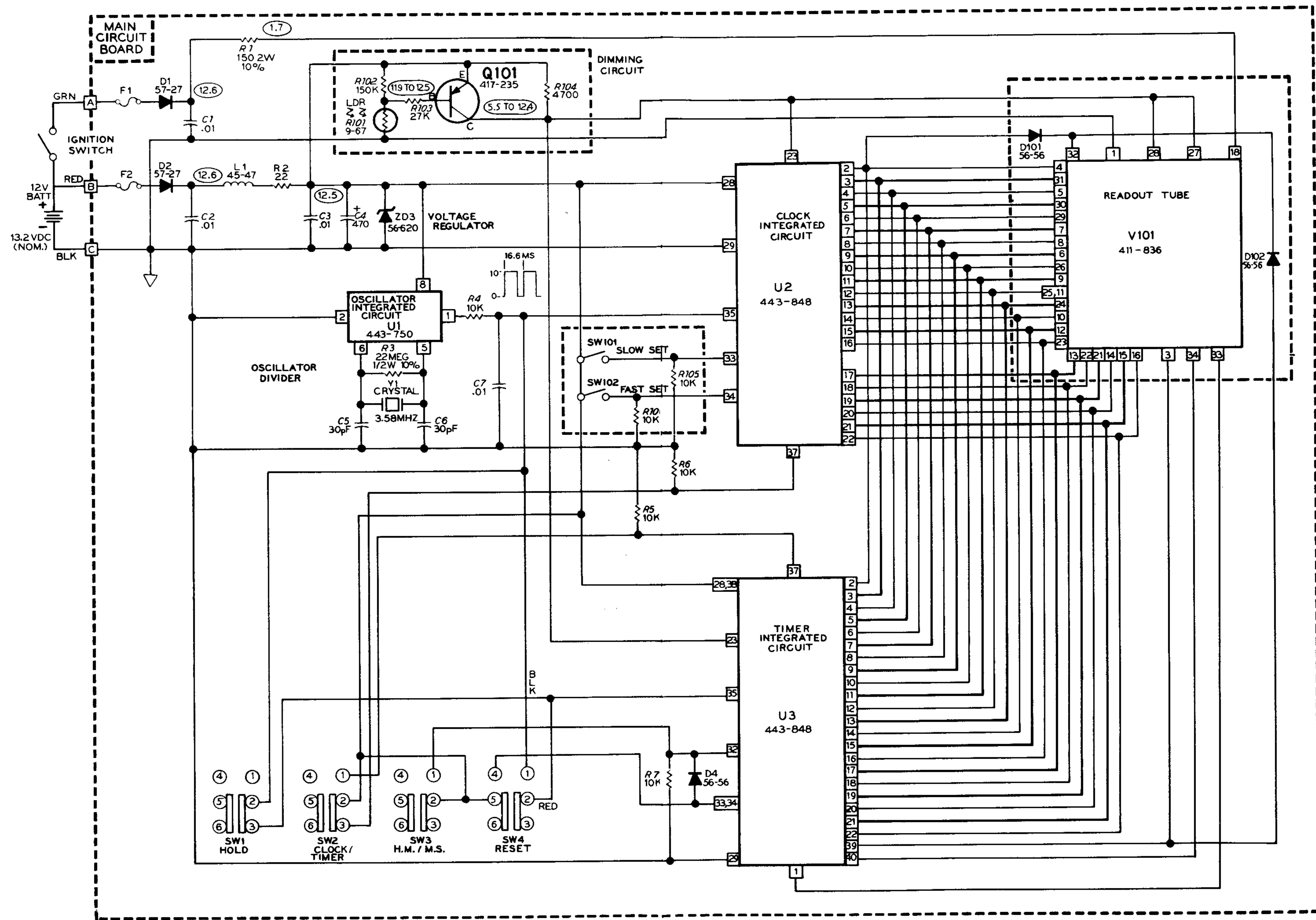
SCHEMATIC OF THE HEATHKIT® QUARTZ CLOCK/TIMER MODEL GC-1415
