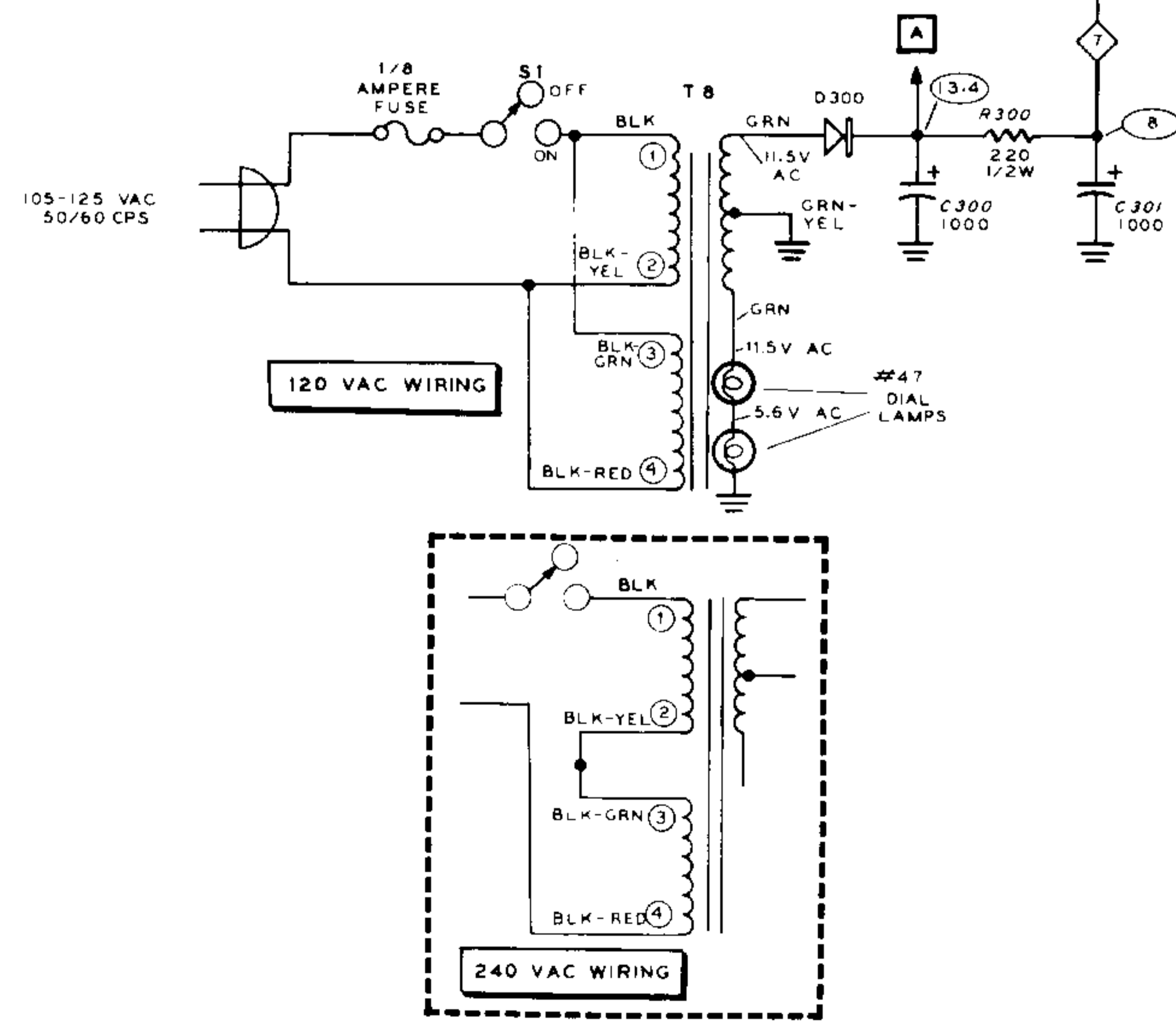
SCHEMATIC OF THE HEATHKIT® SOLID STATE FM STEREO TUNER MODEL AJ-14
